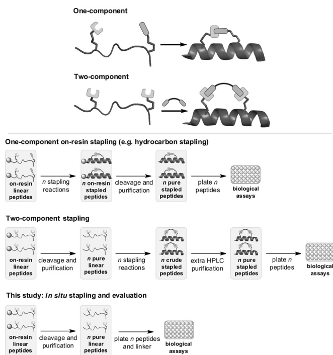
Figure 1. Top: One- and two-component macrocyclization approaches. Bottom: Unlike classical one-component stapling [15] and existing two-component strategies such as our CuAAC method, [7,18] the in situ strategy combines stapling and the primary biological assay in a single step.
