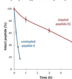
Figure 5. a) Binding affinities by fluorescence polarization (FP). b) MDM2 is stabilized by E1 as shown by cell lysate thermal shift. c) Confocal microscopy of TAMRA-E1 (20 \mu M) in live T22 cells, scale bar: 25 \mu m. Peptide shown in red, nuclei in blue. d) E1 shows increased stability to proteolysis by chymotrypsin.
